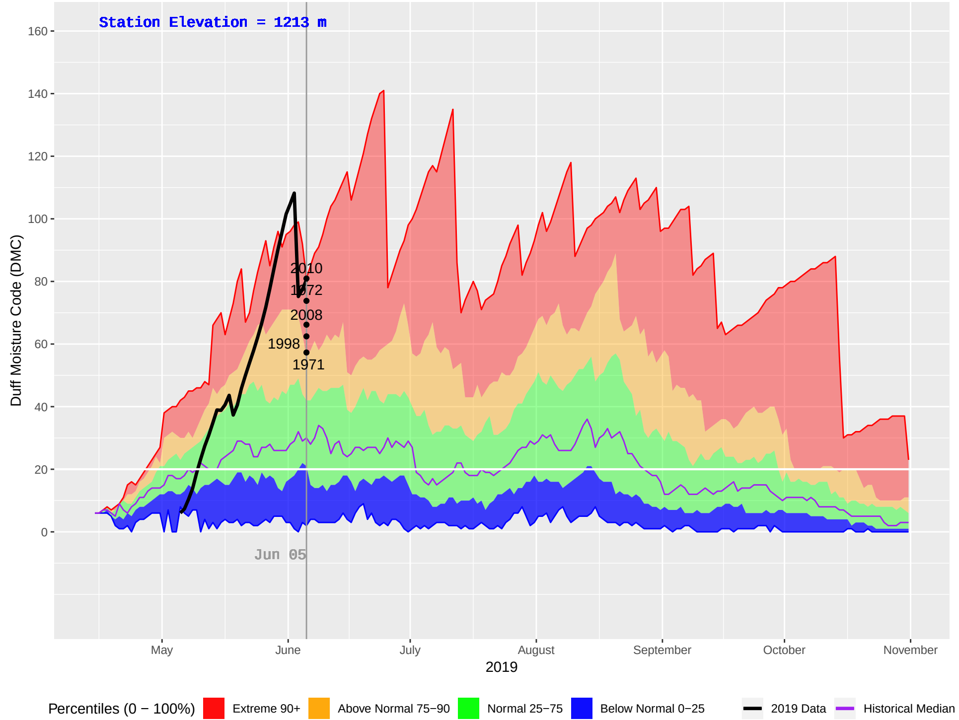
INGENIKA POINT (145) : Historical (1971–2018), Current (2019) Daily Duff Moisture Code (DMC)
