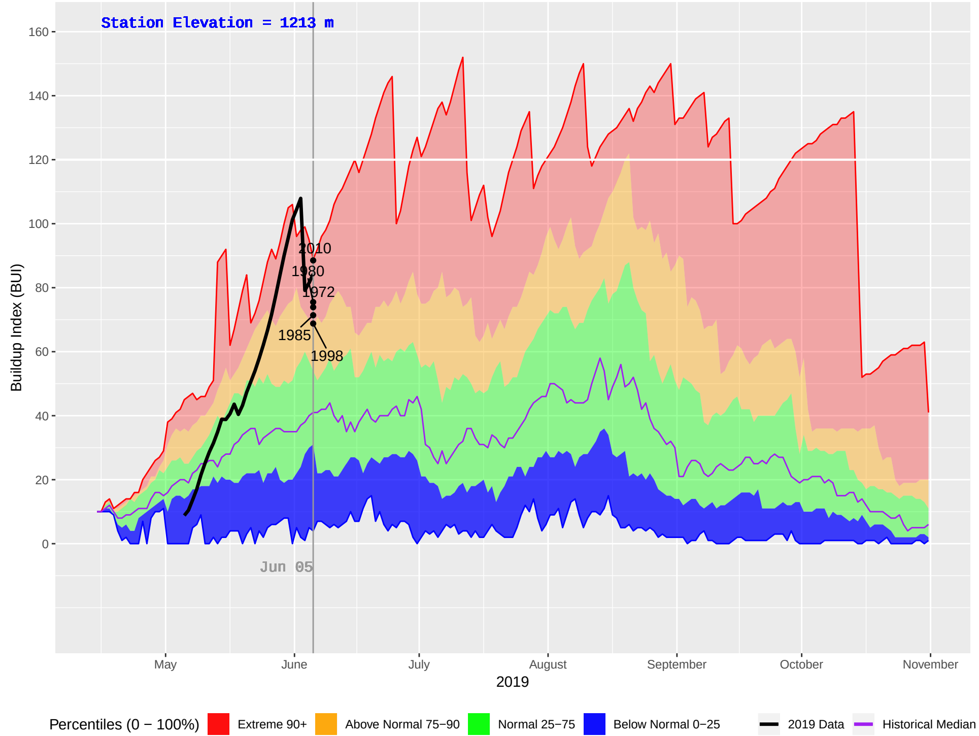
INGENIKA POINT (145) : Historical (1971–2018), Current (2019) Daily Buildup Index (BUI)
