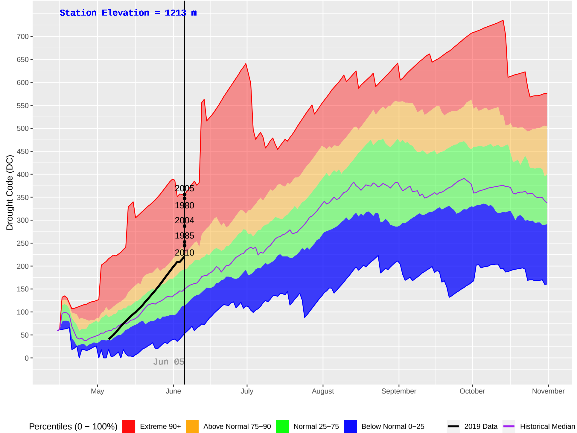
INGENIKA POINT (145) : Historical (1971–2018) and Current (2019) Daily Drought Code (DC)
