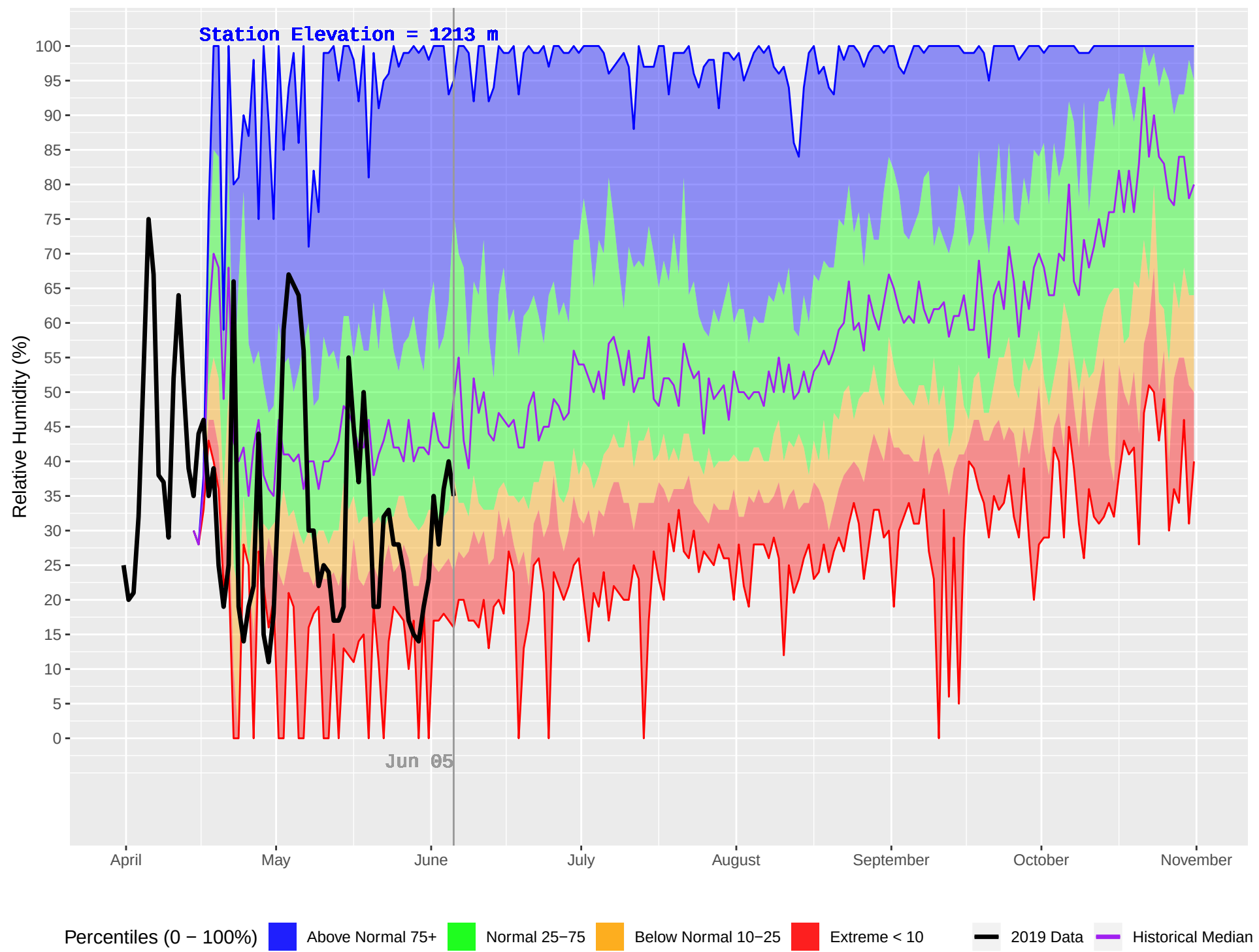
INGENIKA POINT (145) : Historical (1971–2018) and Current (2019) Daily Relative Humidity
